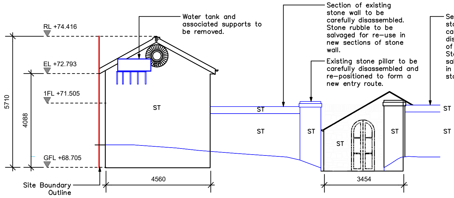
SOUTH ELEVATION
